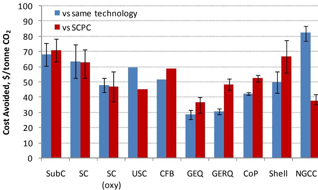
Figure 4: Cost of CO 2 Avoided from Design Studies for Normalised Economic and Operating Parameters for NOAK Plants.
