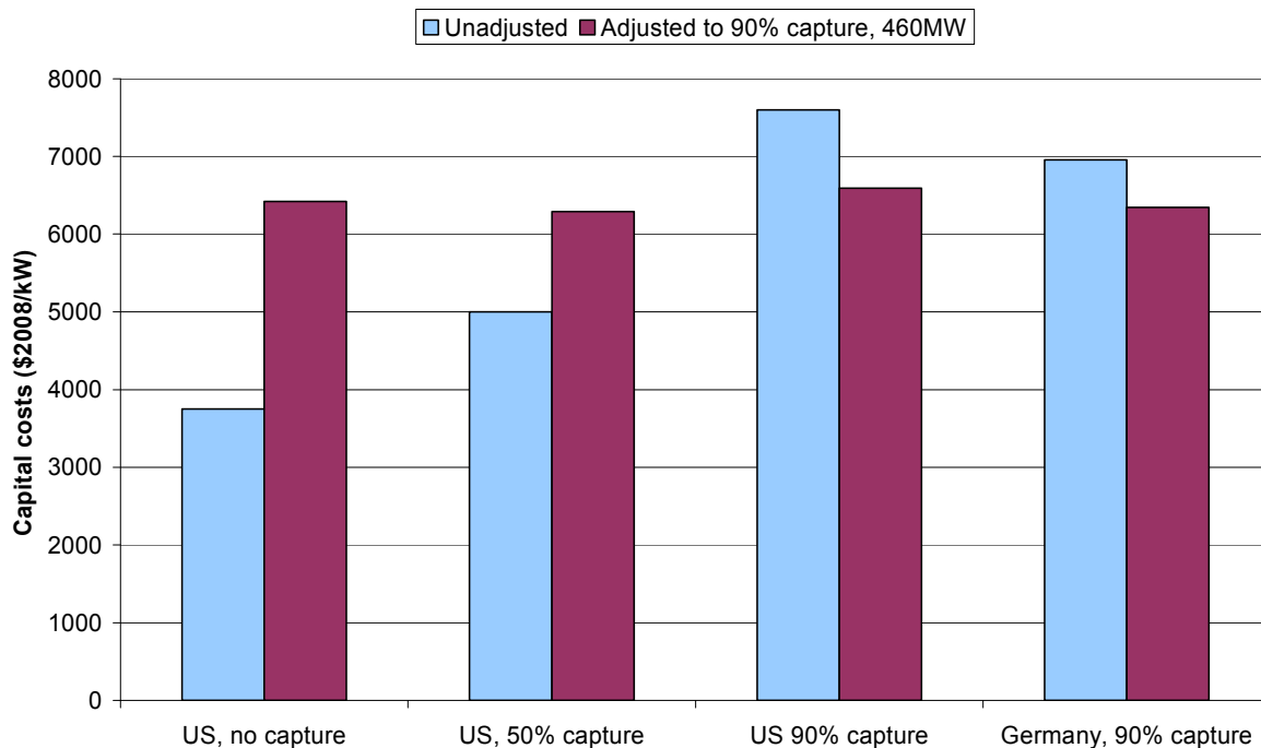
Figure 5: Costs of Early IGCC Plant Adjusted to a Common Basis of 460MW, 90% Capture
